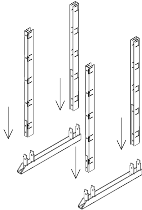
INSTALL VERTICALS FIGURE 9
