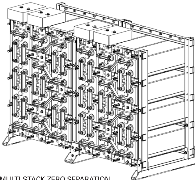
MULTI-STACK ZERO SEPARATION FIGURE 3A
