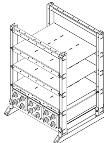
INSTALL MODULES FIGURE 20
