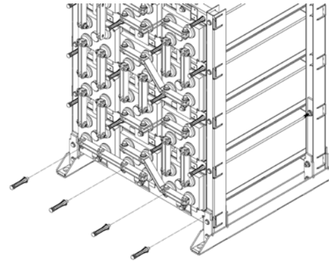
INSTALL SUPPORT POSTS FIGURE 27
