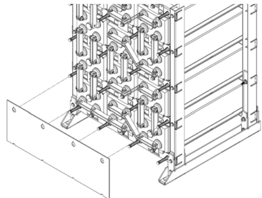
INSTALL SAFETY SHIELDS FIGURE 28
