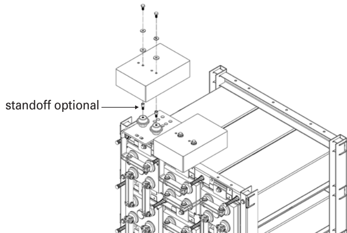
INSTALL TERMINAL PLATE COVER FIGURE 29
